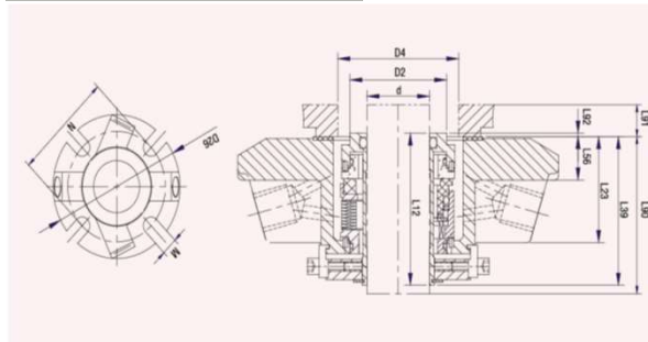
TD-CARTRIDGE SEAL
